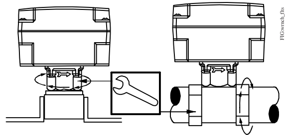
Figure 5: Use Only the Wrench Flats Provided
