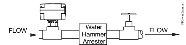
Figure 9: Water Hammer Arrester Location
