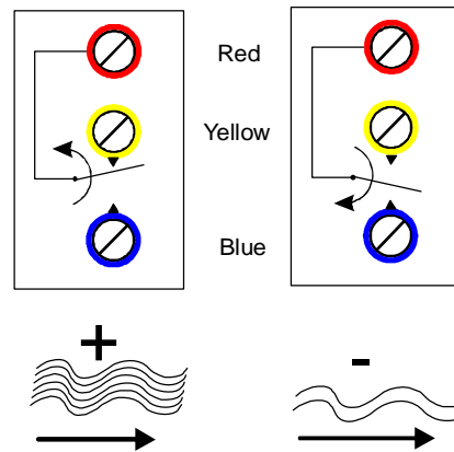
Figure 10: F261 Control Switch Action
