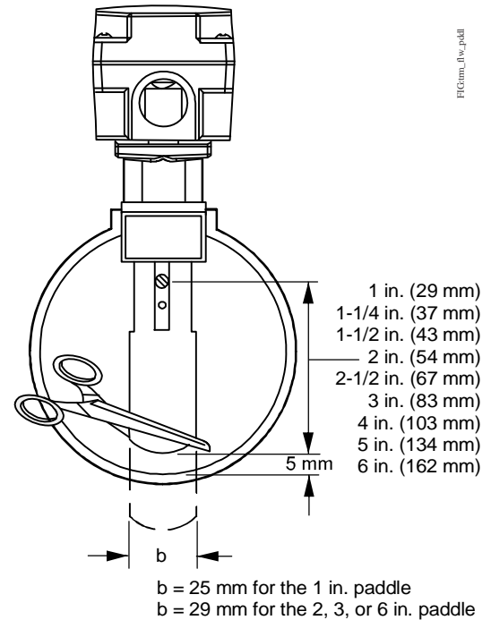
Figure 3: Trimming the Flow Paddles
