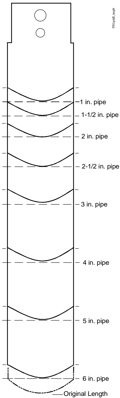
Figure 4: Trimming Diagram for the Large Flow Paddle
