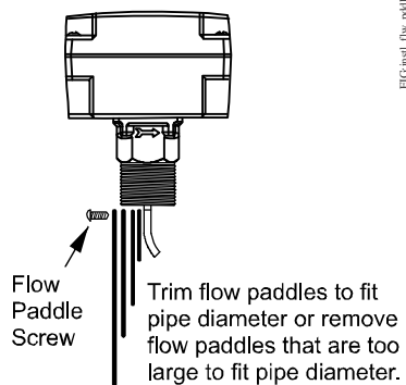
Figure 2: Installing the Flow Paddles
